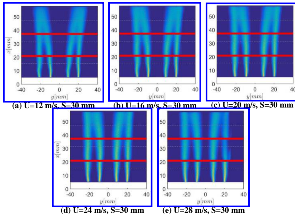
Figure 7: Flame surface density images for Bunsen flames (Flames H-L).
