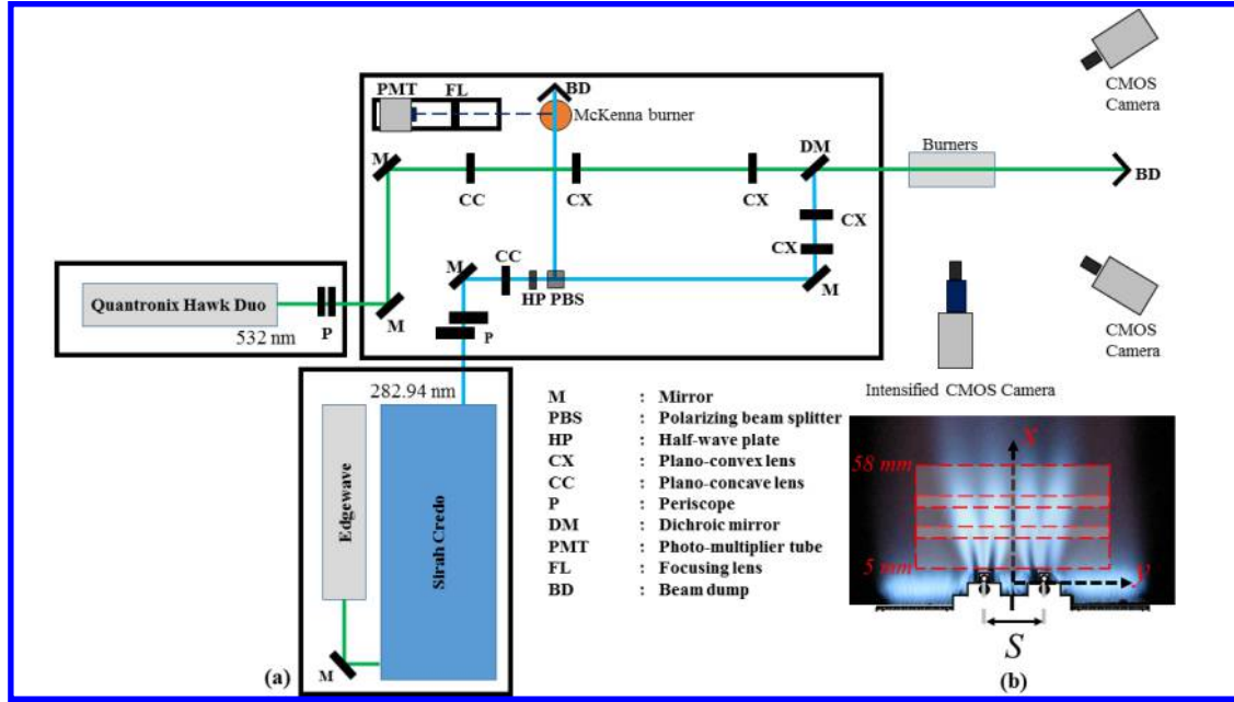
Figure 2: (a) Sketch of the OH-PLIF and s-PIV system (top view), and (b) three FOVs overlaid on top of bluff-body flames with all pilot flames.
