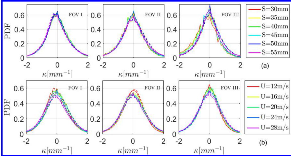
Figure 12: PDF of flame curvatures in the inner (solid) and outer (dashed) branches for (a) bluff-body (A-F), and (b) Bunsen flames (H-L).
